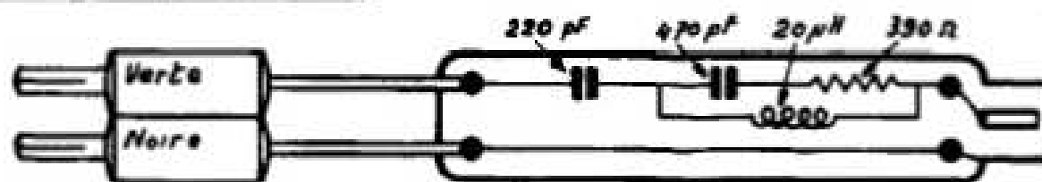
SAF ANTENNE FICTIVE
